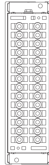
Terminal layout
