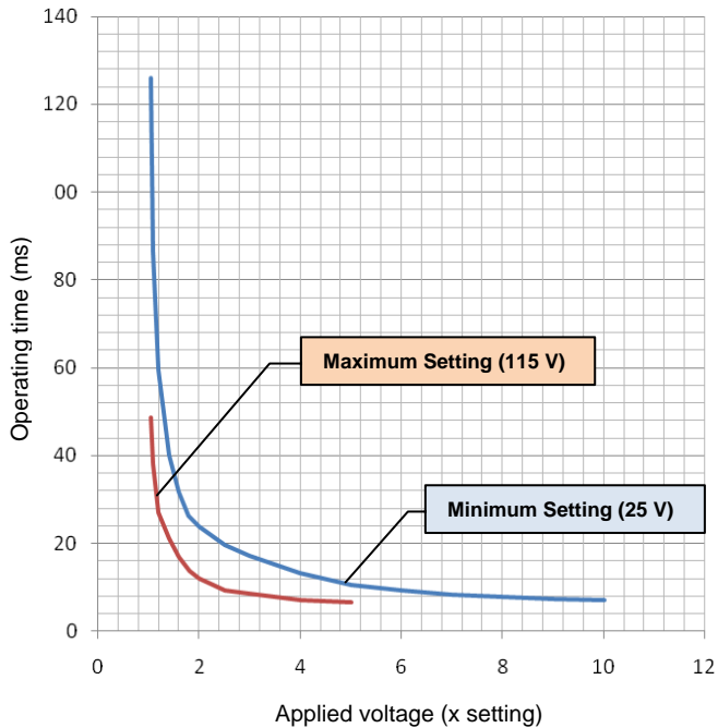
Figure 1 – 2V73 Operating Characteristic
