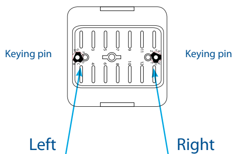
Bottom view relay
